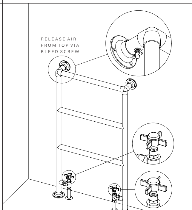
8. RELEASE AIR
