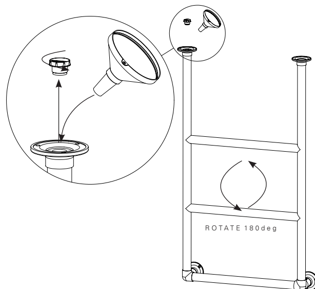
2. FUNNEL PLACEMENT
