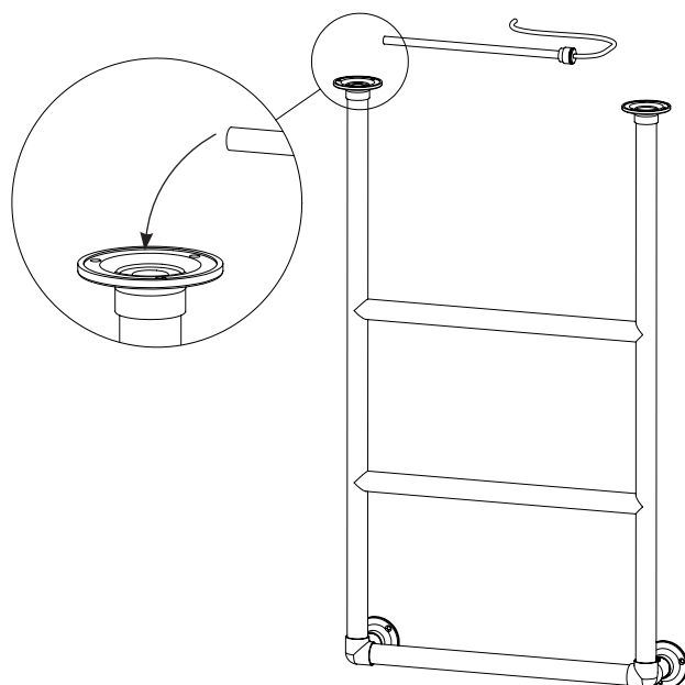
4. ELEMENT ASSEMBLING
