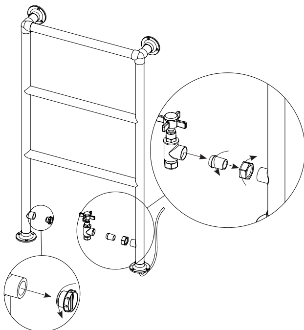
1. PRE-INSTALLATION PLUMBING
