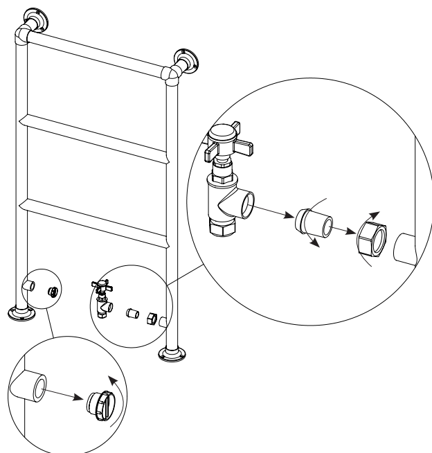
2. VALVES ASSEMBLING
