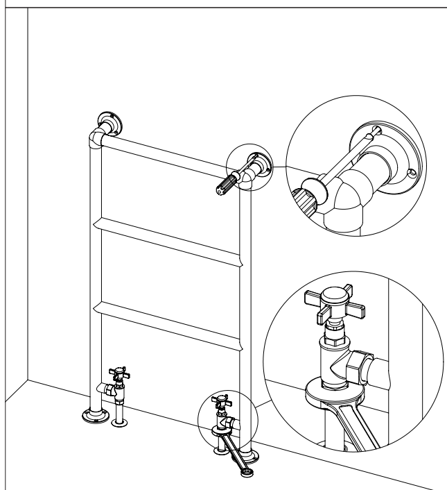
7. FIXING TOWEL RAIL
