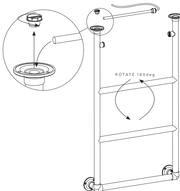
2. ELEMENT ASSEMBLING
