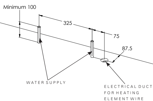
1. PRE-INSTALLATION PLUMBING
